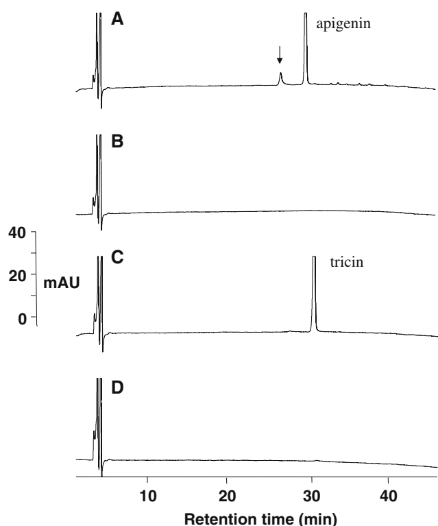
Fig. 6 HPLC chromatograms of extracts of incubation mixtures of mouse liver microsomes with NADPH and apigenin ( a ) or tricetin ( c ) (both at 100 \mu M) or without flavones ( b , d ). Duration of incubation was 30 min. The chromatograms are representative of two experiments using pooled microsomes from three mice. Arrow marks metabolite peak. Control incubations omitting NADPH afforded chromatograms identical to those shown in b and d (in which flavones were omitted). AU absorbance units. Chromatographic analysis was conducted using the Varian system (gradient elution); thus, retention times are different from those shown in Fig. 3. For conditions of incubation and chromatography see Materials and methods
