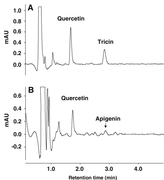
Fig. 2 HPLC chromatograms of plasma from mice, which had ingested tricin ( a ) or apigenin ( b ) at 0.2% for a week in their diet. Each chromatogram is representative of four mice. Quercetin served as internal standard. AU absorbance units. Chromatographic analysis was conducted using the Acquity system in isocratic elution mode, for conditions see Materials and methods. The retention times of tricin and apigenin in spiked samples were 2.84 and 2.83 min, respectively, thus not identical, but very close to each other. On further chromatographic investigation using several conditions allowing increased retention times, the peaks just after the solvent front in b did not co-elute with apigenin conjugates
