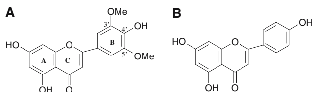
Fig. 1 Chemical structure of tricetin (a) and apigenin (b)
