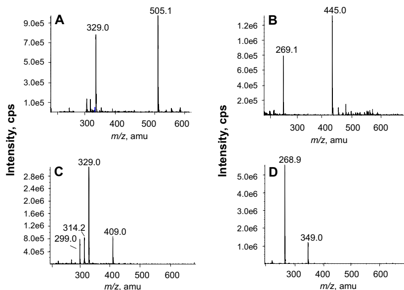
Fig. 4 On-line HPLC–MS mass spectra of metabolite peaks in extracts of incubates with human liver microsomes ( a, b ) or cytosol ( c, d ) including tricetin ( a, c ) or apigenin ( b, d ). Each spectrum is representative of six samples from pooled preparations from three humans. HPLC separation was achieved using the Varian system. The separation of the glucuronide peaks was not as satisfactory as that shown in Fig. 3 using the Acquity system; there-
